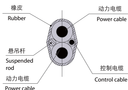
电缆绑扎示意 Picture of cable bundle
